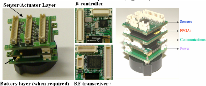
Fig. 1. Tyndall25 modular platform
